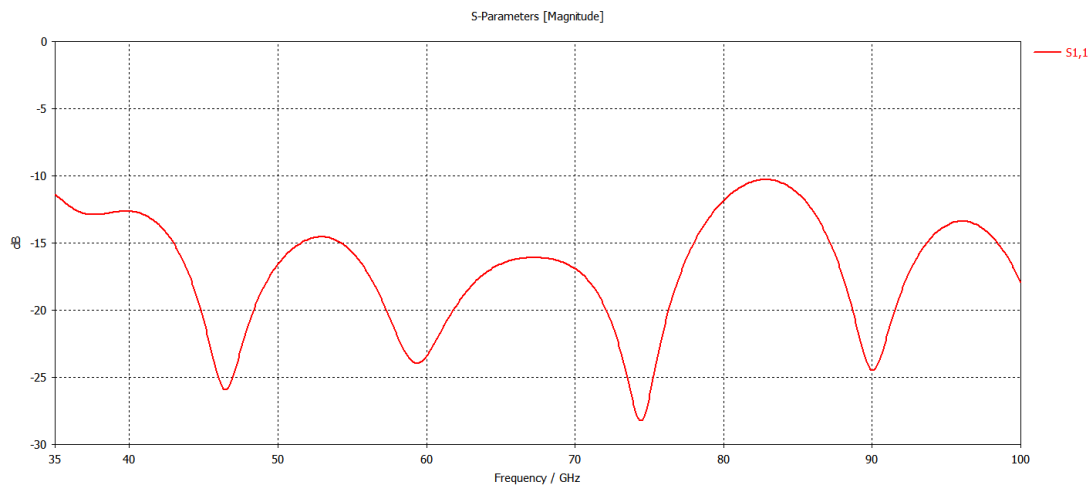
Figure 3. Simulated return-loss ( S_{11} ) characteristics of the proposed antenna.
