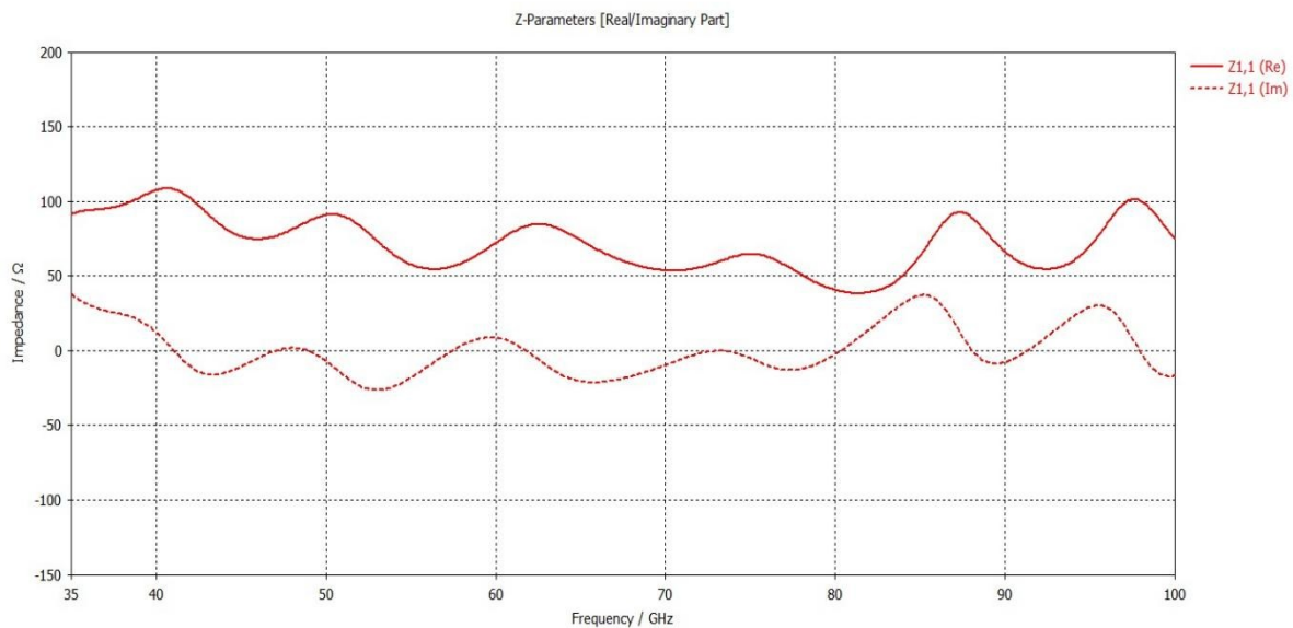
Figure 5. Input Impedance of proposed Antenna.
