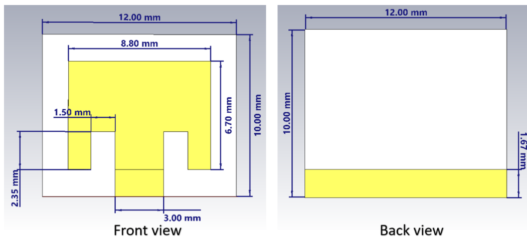
Figure 1. Design layout of the proposed antenna
