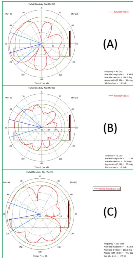
Figure 6 (A-C). Simulated 2D far-field radiation patterns of the antenna
