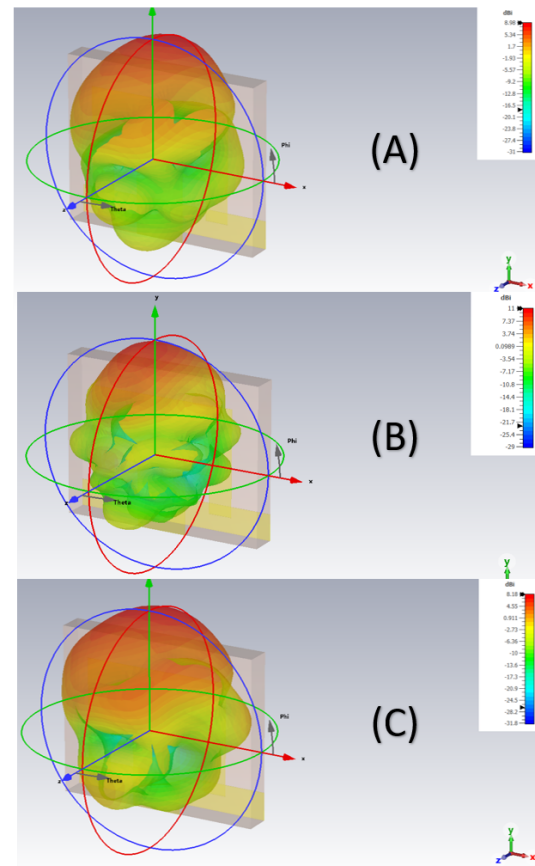
Figure 7(A-C) 3D far-field radiation patterns of the antenna
