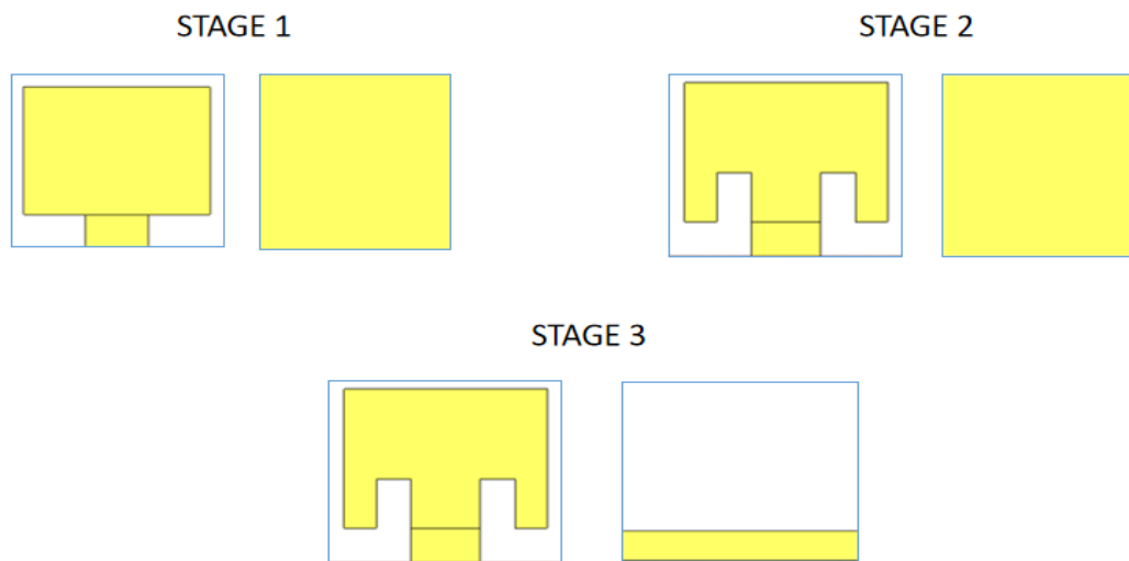
Figure 2. Evolution stages of the proposed antenna
