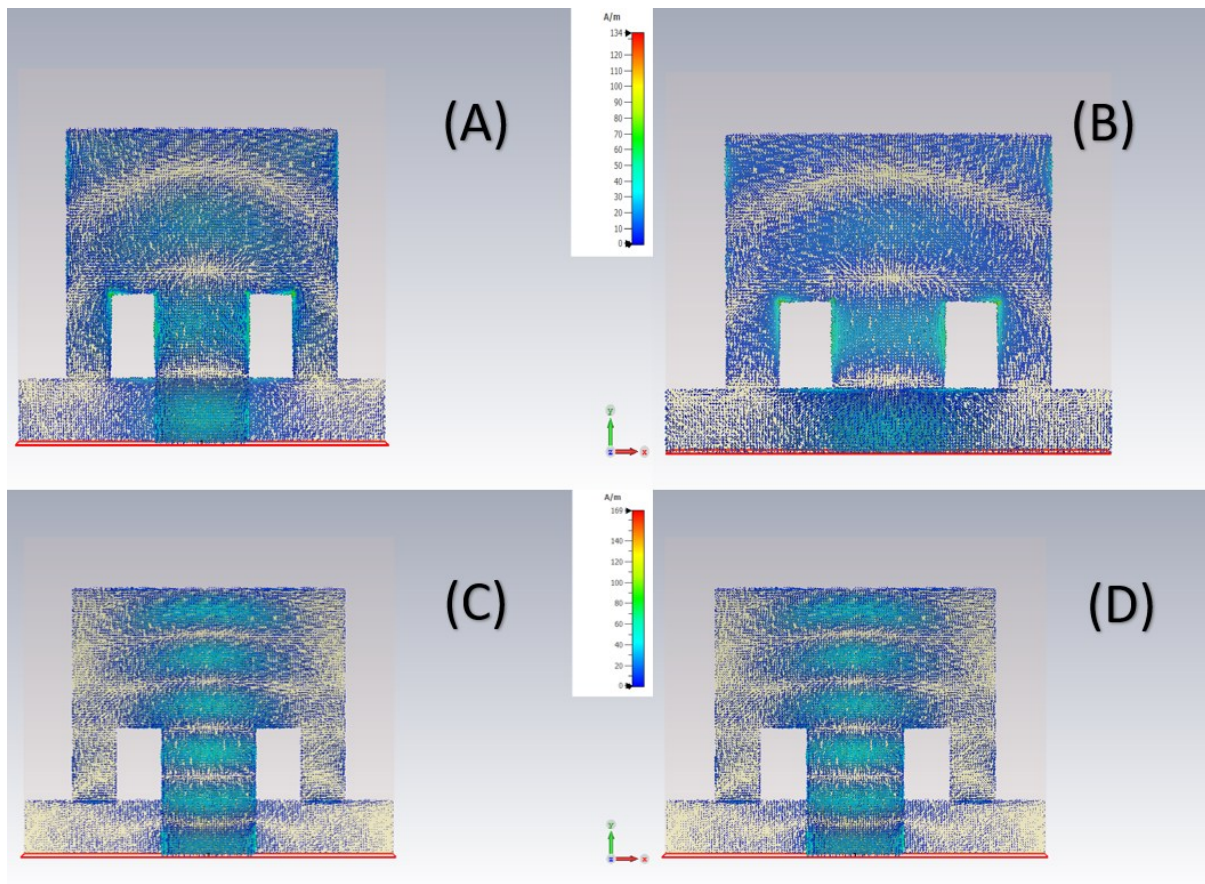
Figure 8. (A&B) front and back view of surface current distribution at 45 GHz, (C&D) front and back view of surface current distribution at 75 GHz.
